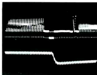
Fig. 16 Vertical-blanking section of negative-going video compared to a vertical deflection pulse (left photo) shows why such a narrow pulse (when used to supplement the vertical blanking in older color sets) did not blank out the entire retrace period. Picture at right shows the video and the yoke current during retrace. Only yoke current drops when retrace occurs.
